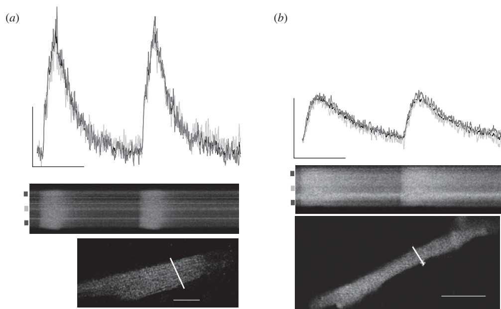
Figure 2. Spatial and temporal cellular \text{Ca}^{2+} flux in ventricular myocytes from thermally acclimated Pacific bluefin tuna. Representative time courses (top) and corresponding raw line scan images (below) show temporal and spatial characteristics of \text{Ca}^{2+} flux in a (a) CA and (b) WA myocyte. Markings on left side of line scan images show regions (cell centre, light grey lines; cell periphery, dark grey lines) for spatial characterization (see electronic supplementary methods for details). The time course of the \text{Ca}^{2+} transient across the whole width of the cell is given by the black time course line, which is partially obscured by the overlapping time courses at the cell centre and periphery. Images below the line scans show the corresponding myocyte loaded with Fluo-4 AM. The white line indicates position of scan. The white scale bar is 20\ \mu\text{m} in both images. Time course scale is 100\ \text{nM} [\text{Ca}^{2+}] by 1\ \text{s} . Line scans are 2500\ \text{lines} \times 512\ \text{pixels} .
